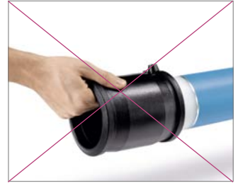
Fig. 72 Do not touch the inside of the electrofusion fitting.
