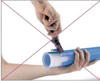
Fig. 69 Do not scrape beyond the markings.
