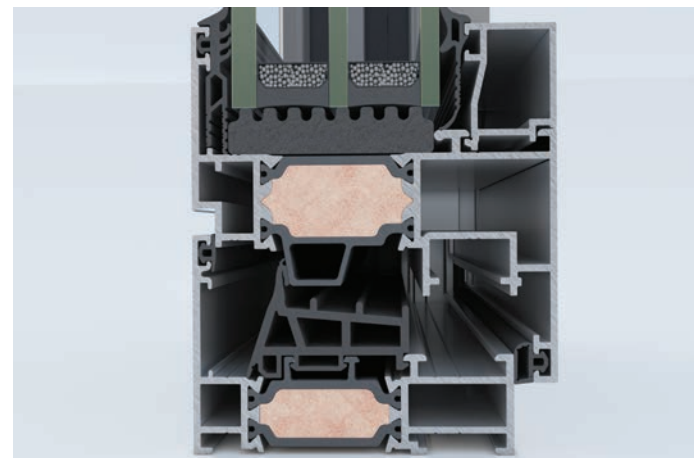
ELVIAL I 2 _ INNOVATIVE INSULATION TECHNOLOGY FOAM INSULATING PROFILE & GLAZING GASKETS WITH FINS
